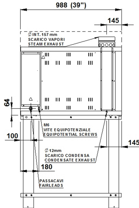
REAR VIEW
